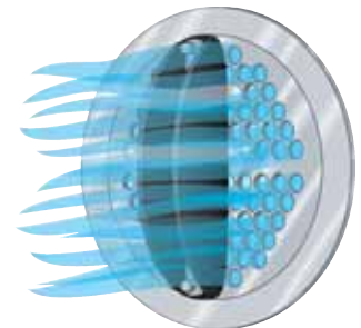
Reverse pressure seals the elastomer disk against the plate, preventing backflow.
